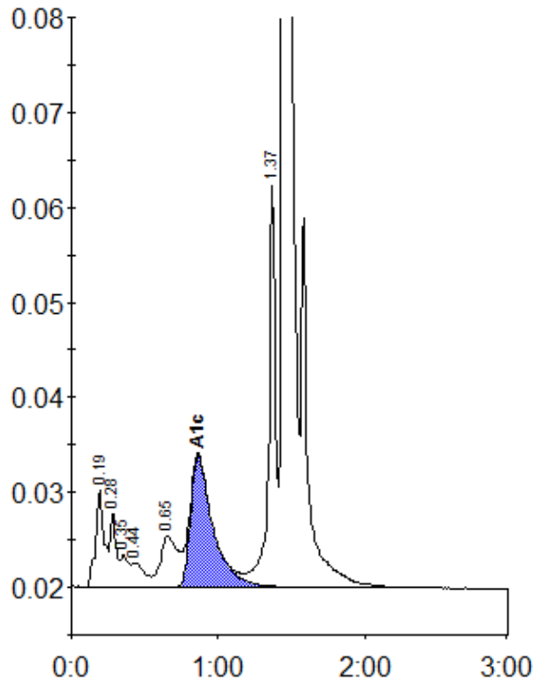
Peak table - ID: 10418176
